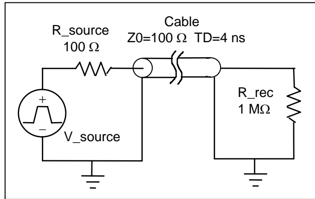
Figure 82 - A transmission line with perfect source termination
