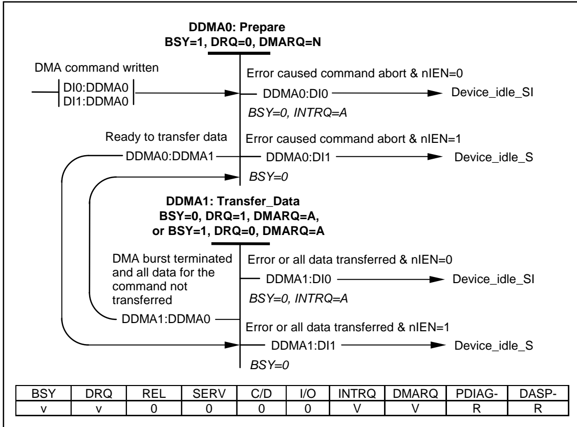
Figure 52 – Device DMA state diagram
