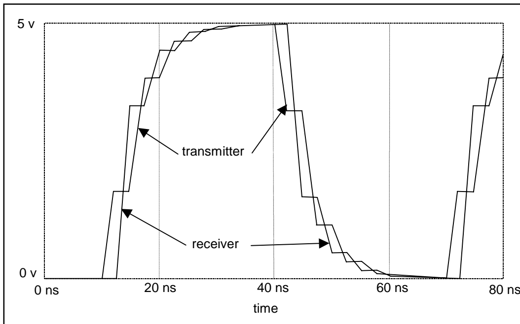
Figure 86 - Waveforms on a source-terminated bus with R_{source} greater than cable Z_0
